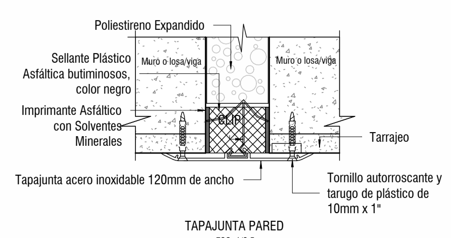
TAPAJUNTA PARED
