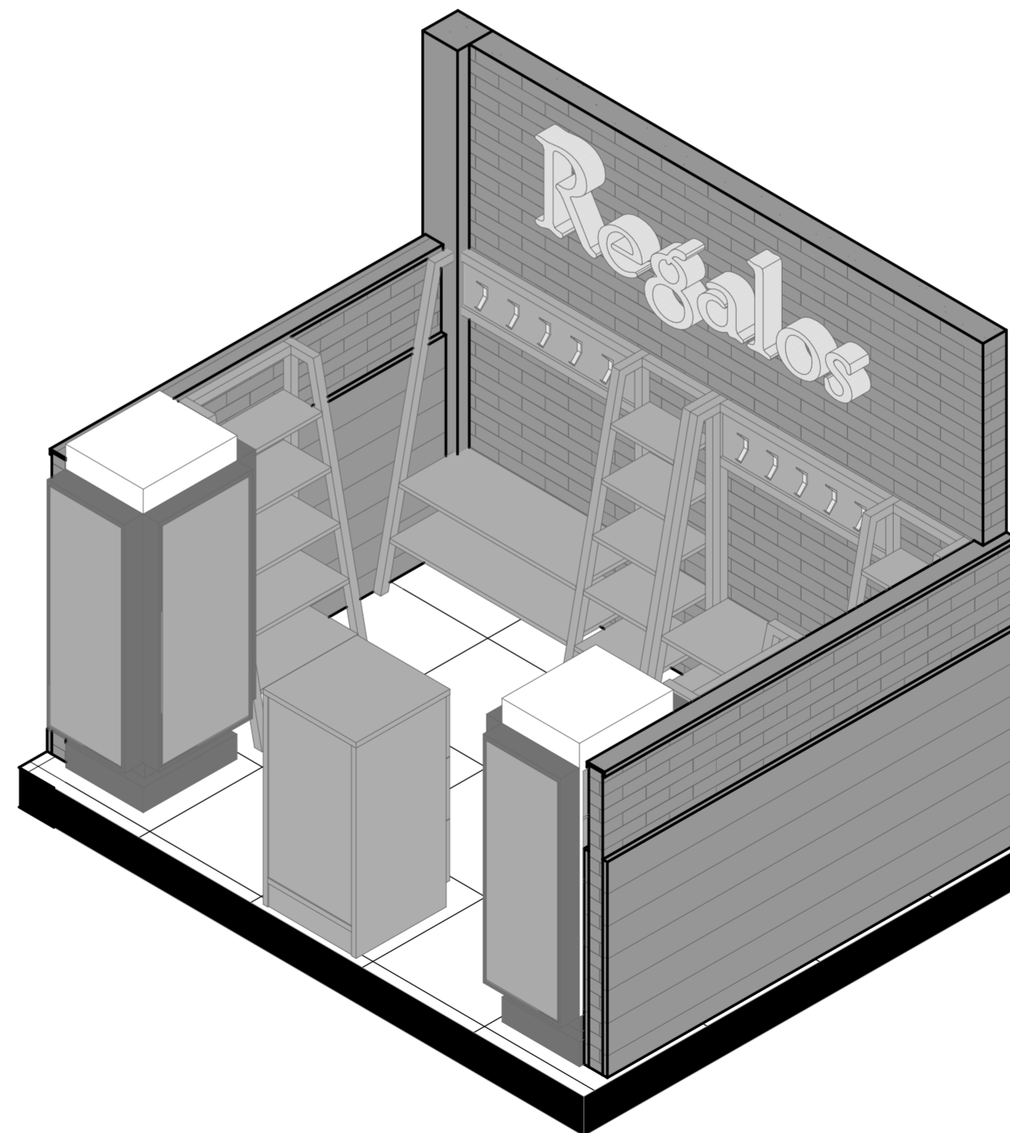
3D-17 ISOMETRIA Esc: 1:25
