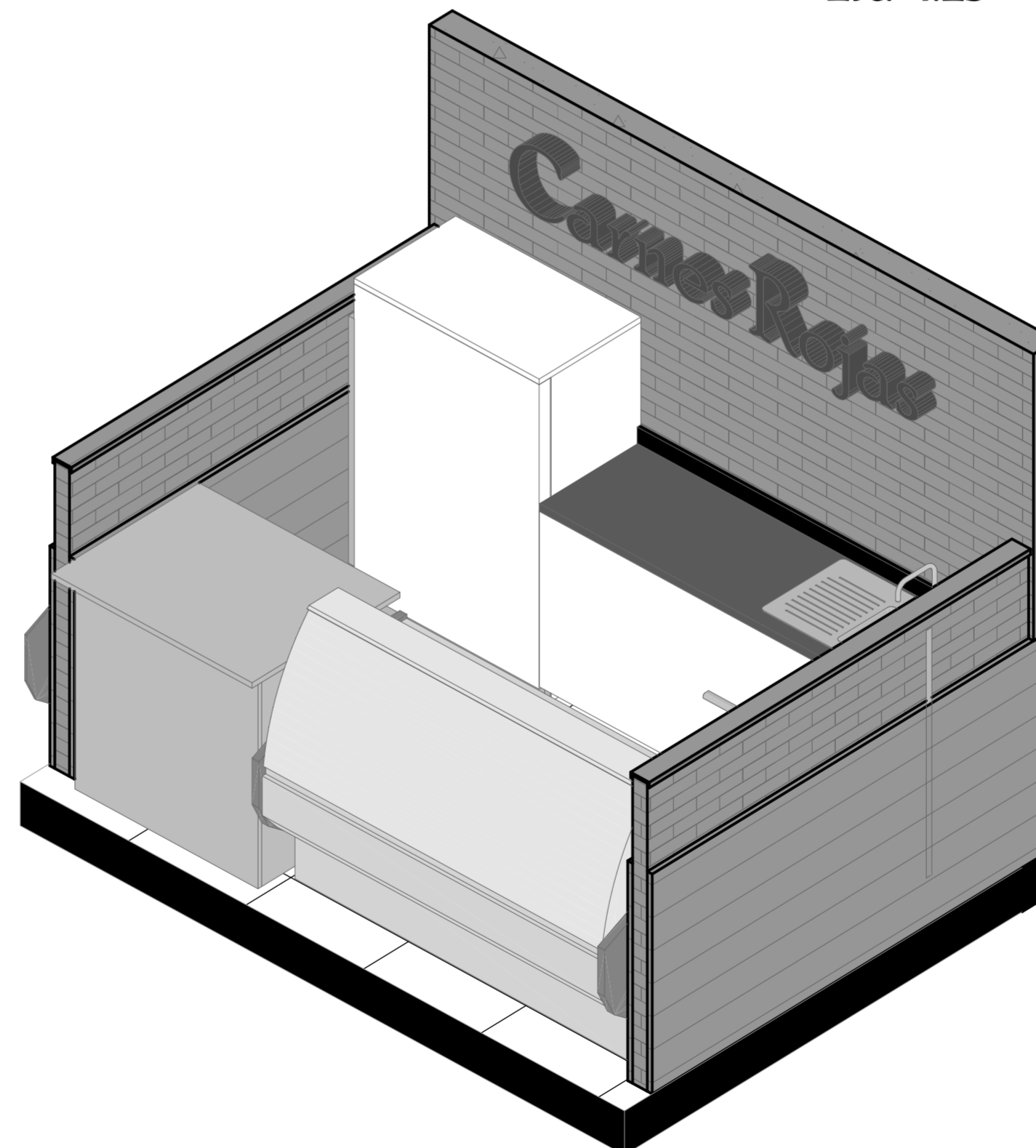
3D-02 ISOMETRIA Esc: 1:25
