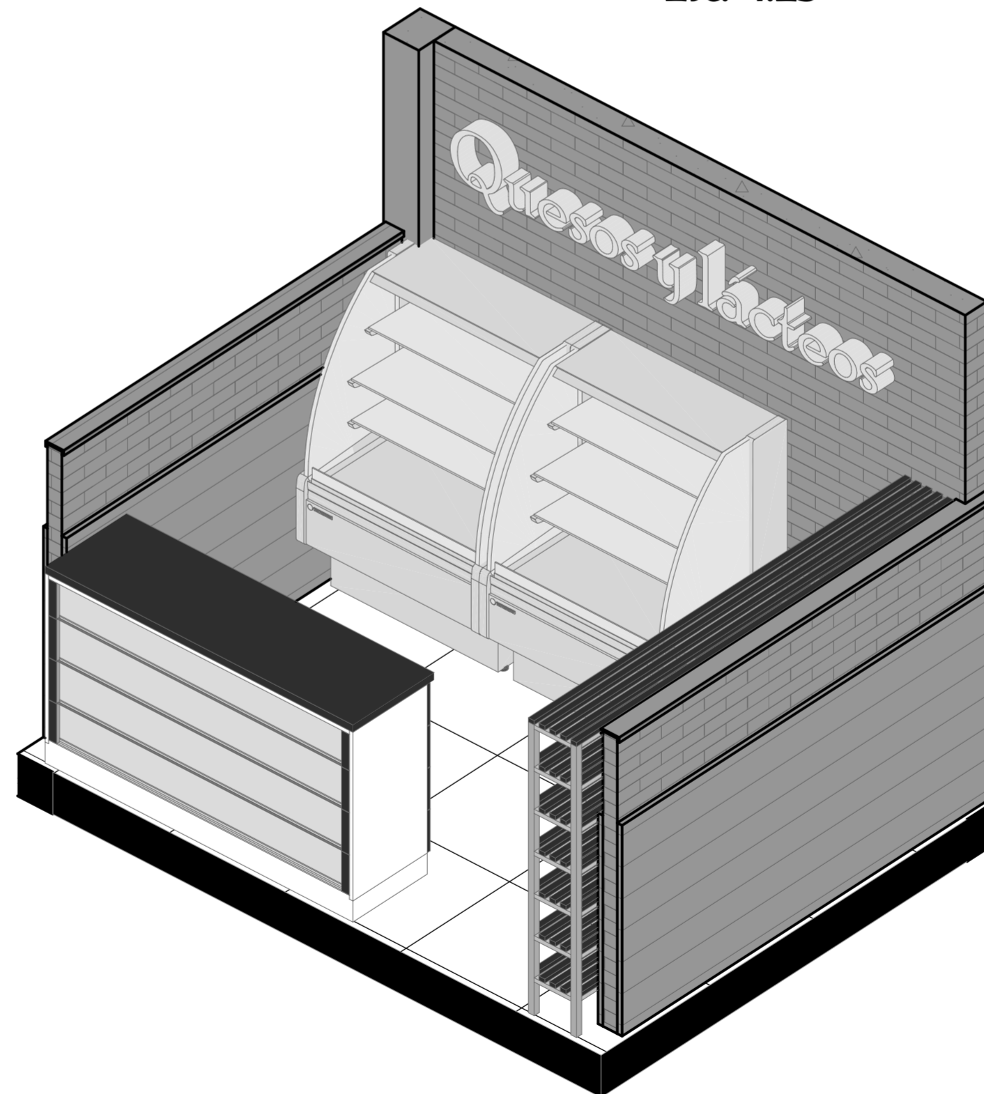
3D-05 ISOMETRIA Esc: 1:25
