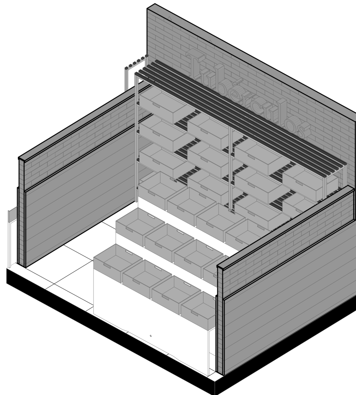
3D-04 ISOMETRIA Esc: 1:25
