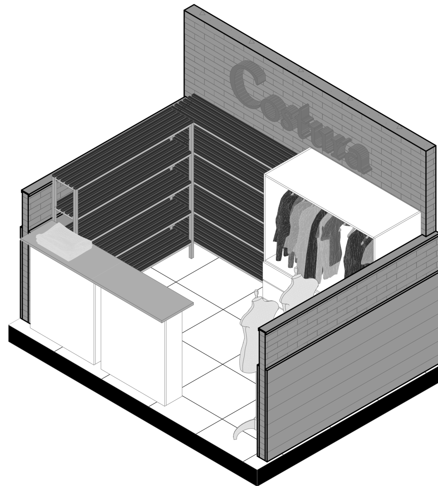
3D-14 ISOMETRIA Esc: 1:25
