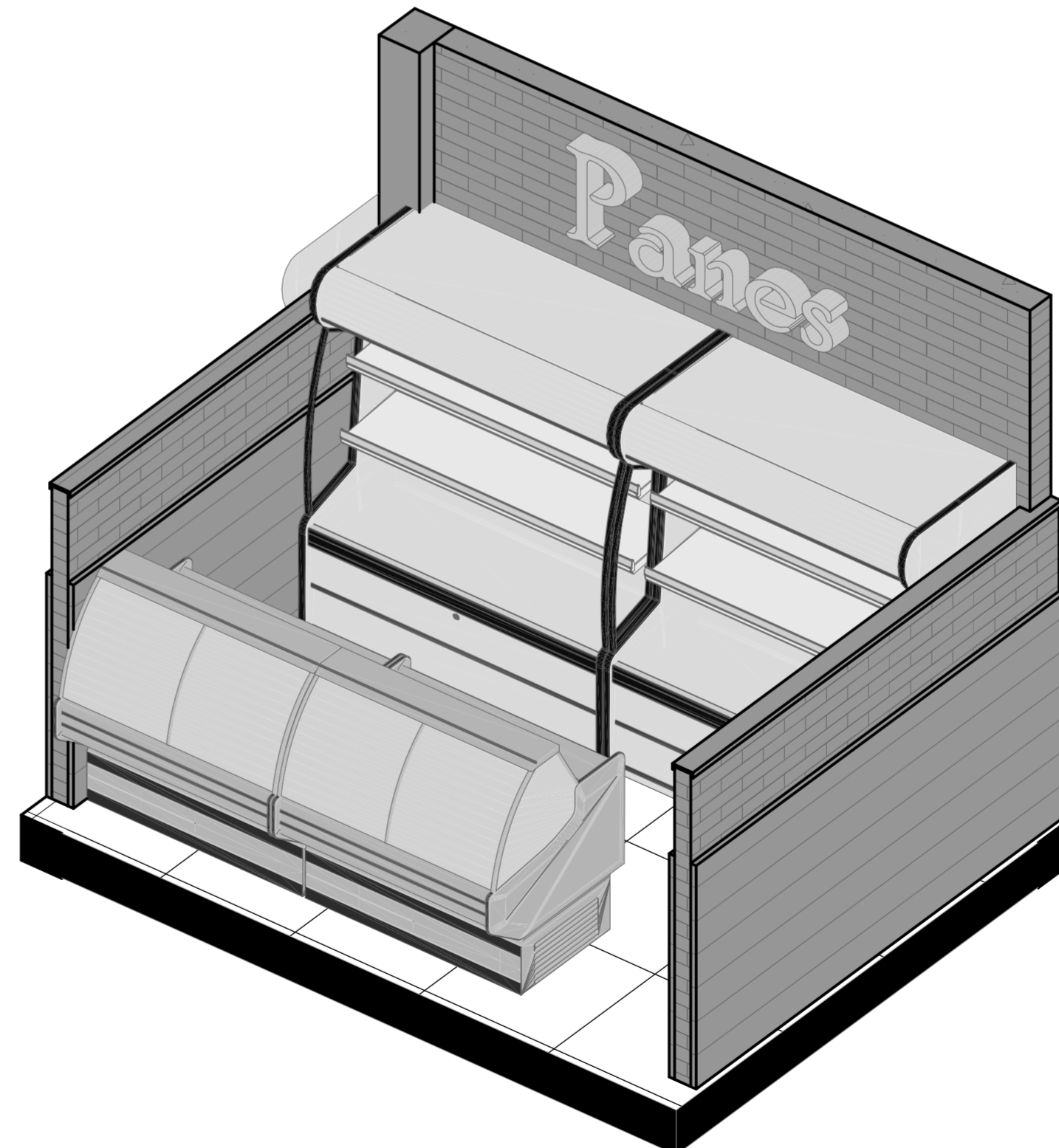
3D-08 ISOMETRIA PANES Esc: 1:25
