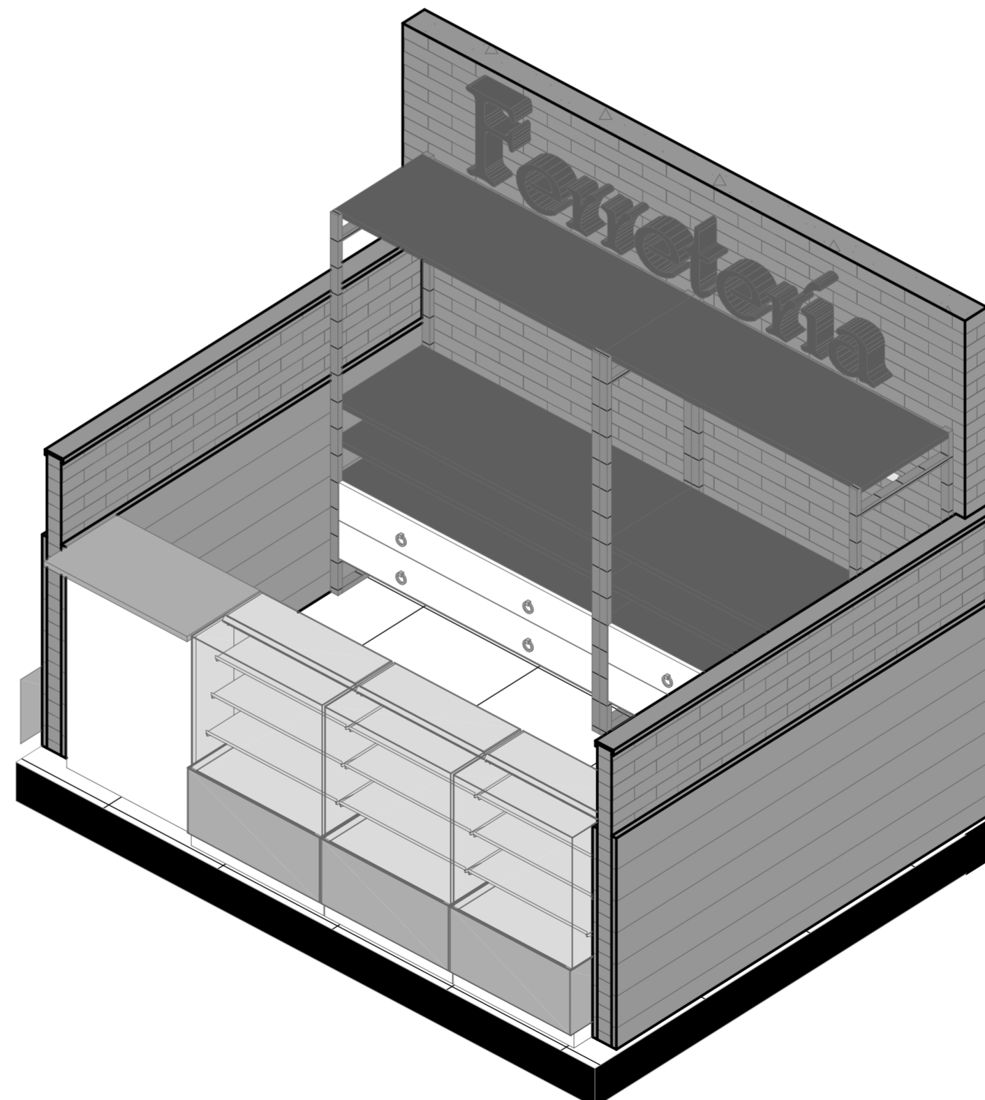
3D-13 ISOMETRIA FERRETERIA Esc: 1:25
